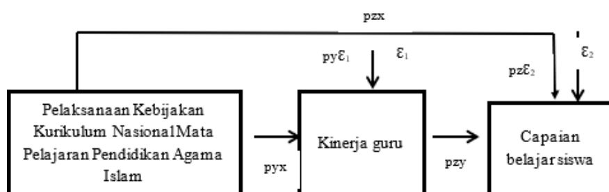
Gambar 1. Paradigma Penelitian
